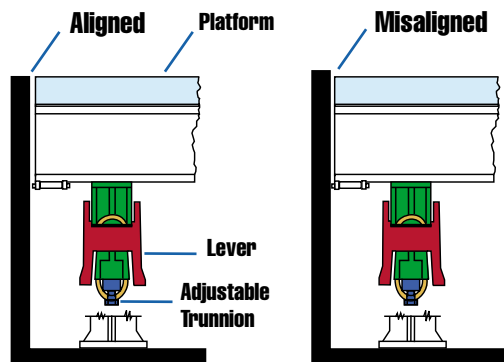
Platform alignment by adjusting Trunnion bolts
